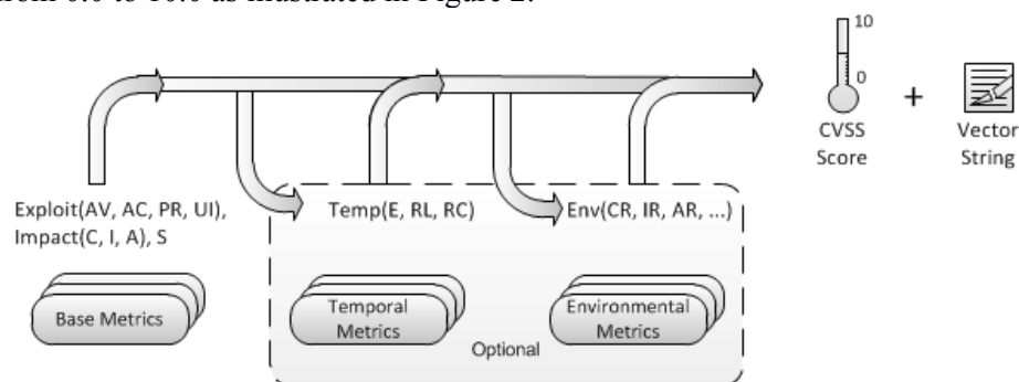
Figure 2: CVSS Metrics and Equations
